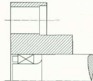
Fig. 4 : Coupling half mounted with GSN 7012 locking assembly.
