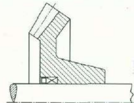
Fig 6 : Bevel gear mounted using GSN 7012 locking assembly. The locking assembly transmits both the torque and the tooth pressure axial component.
