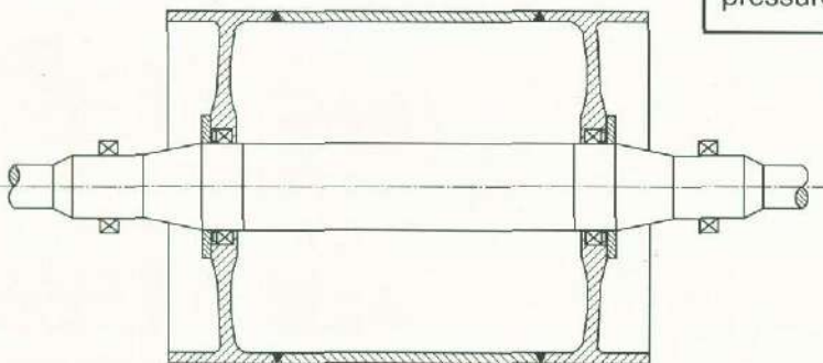
Fig 7 : Belt drum mounted with GSN 7012 locking assemblies.
