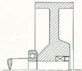
Fig. 5 : Flywheel mounted using one GSN 7012 locking assembly.
