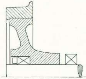
Fig. 3 : Track wheel mounted using GSN 7012 locking assembly.
